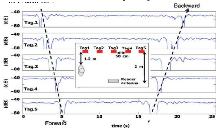
Fig. 7. Backscattered power variation from a linear cluster of tags attached on the wall during the walk of a subject into a corridor. The sequence of the nulls carries information about the direction of motion (delays among nulls) and velocity (slope of the enveloping line through the nulls).
