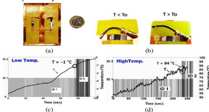
Fig. 3. (a) Two-chip (with ID1 and ID2) temperature threshold sensor integrating a Nitinol switch [13]. (b) Switch closed (chip is inactive, only ID1 is transmitted) and open (chip is active depending on the temperature, ID2 is transmitted in addition to ID1). (c) Chips' responses versus temperature for 0 °C-threshold Nitinol. (d) Chips' responses versus temperature for
