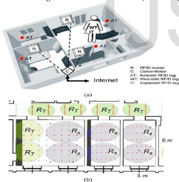
Fig. 1. (a) Sketch of an RFID-powered habitat with ambient tags (AT) attached over the walls and objects, wearable tags (WT), and implanted tags (IT) placed over and inside the human body, one or more RFID readers (R) scanning the rooms and a wireless concentrator (C) capable to pack the collected data for in-house processing and/or for internet streaming. (b) Example of RFID coverage [2] of a home-portion by a multiplicity of readers' antennas placed at the walls' side ( R_s ) and over the top ceiling ( R_T ).
