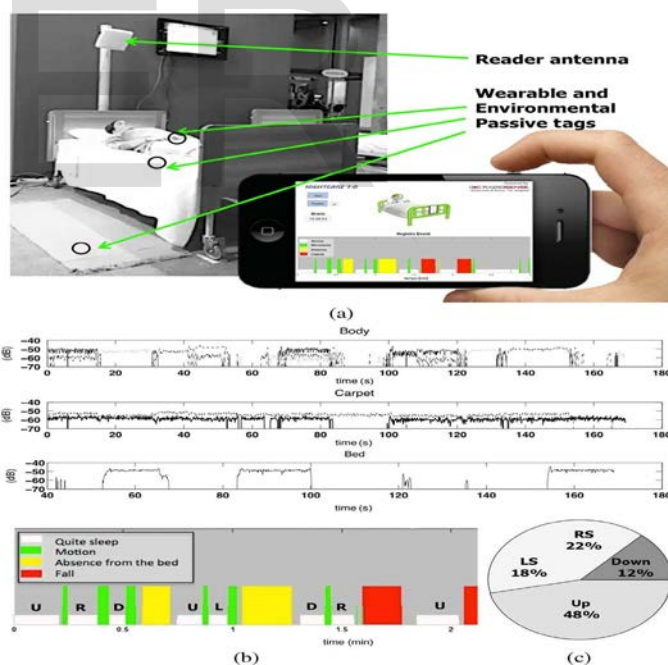
Fig. 9. (a) Ambient intelligence system aimed to take care of the night sleep involving RFID tags placed over the body and in the surrounding environment.
