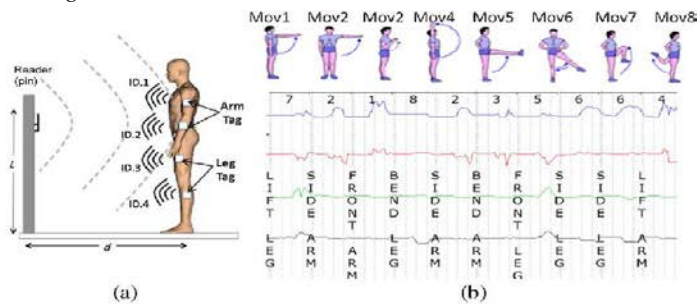
Fig. 8. (a) Set-up as in [31] for the classification of arms and leg gestures by passive RFID ( d = 1.2\text{ m} ; L = 0.9\text{ m} ). (b) Examples of RFID backscattered patterns to be classified by the SVM algorithm performing data mining.
